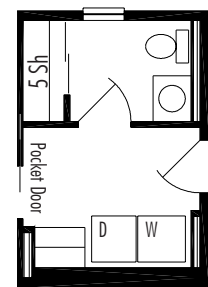
AXU3 Utility Option (Basement Plan Only)
