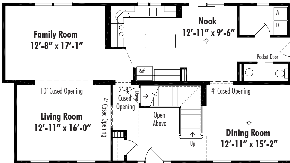
Alexandria I. 48/50 Basement 27'-4" x 48/50', Total Living Area 2592 Sq. Ft.
