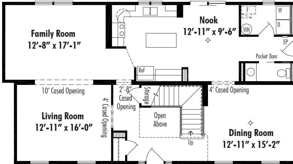
Alexandria I. 48/50 Crawl Space 27'-4" x 48/50', Total Living Area 2592 Sq. Ft.
