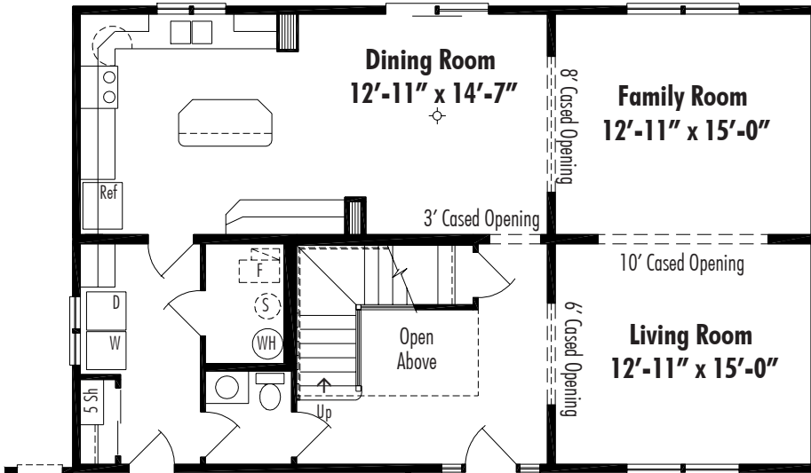
Saratoga I .44 Crawl 27'-4" x 44', Total Living Area 2318 Sq. Ft.
