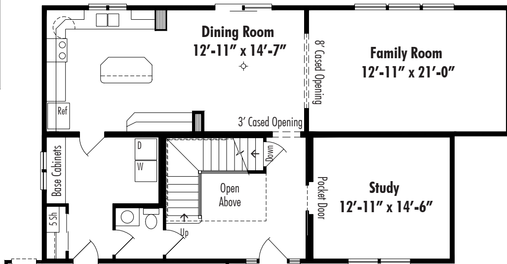
Saratoga II. 44/50 Basement 27'-4" x 44/50', Total Living Area 2400 Sq. Ft.
