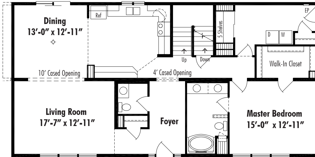
Berkshire .54 Basement 27'-4" x 54', First Floor Living Area 1476 Sq. Ft.
