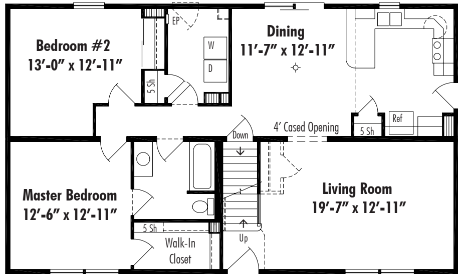
Dover .46 Basement 27'-4" x 46', First Floor Living Area 1257 Sq. Ft.
