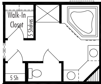
RPB2 Roman Tub and 4' Shower (Requires 6' Extension to Rear of Module)
