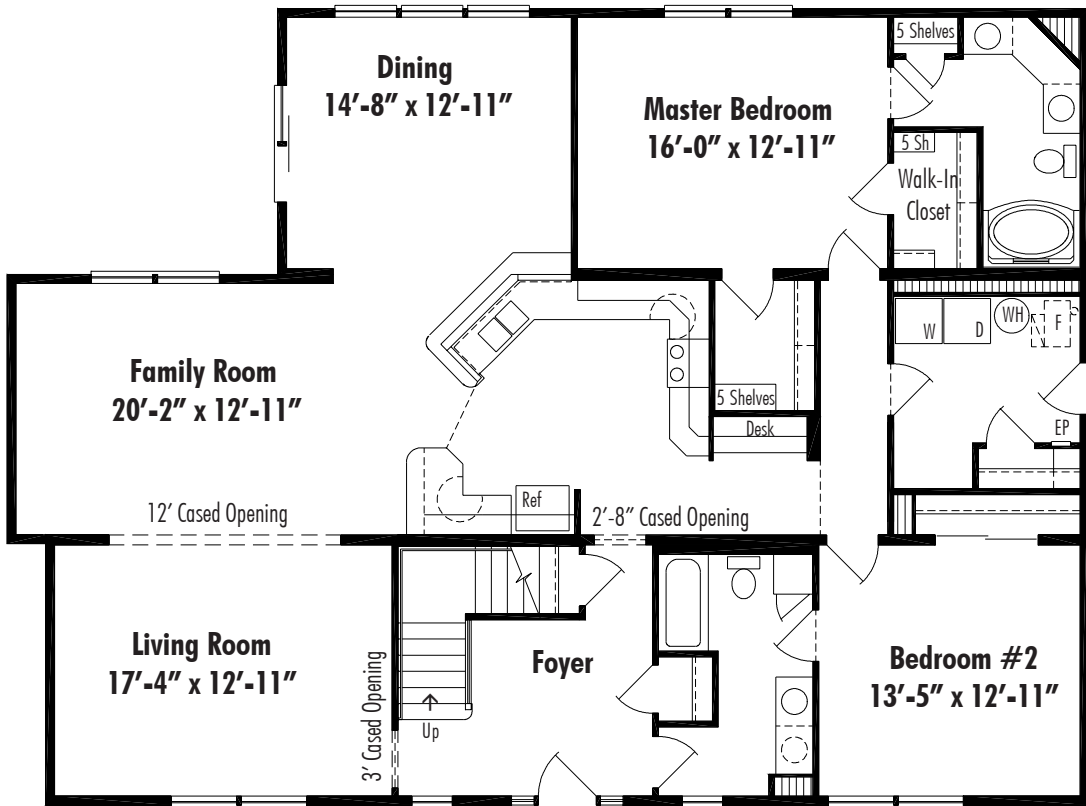
Rockport.54/56 Crawl Space 41' x 54'/56', First Floor Living Area 2077 Sq. Ft.
