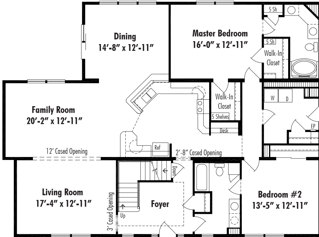
Rockport.54/56 Basement 41' x 54'/56', First Floor Living Area 2077 Sq. Ft.
