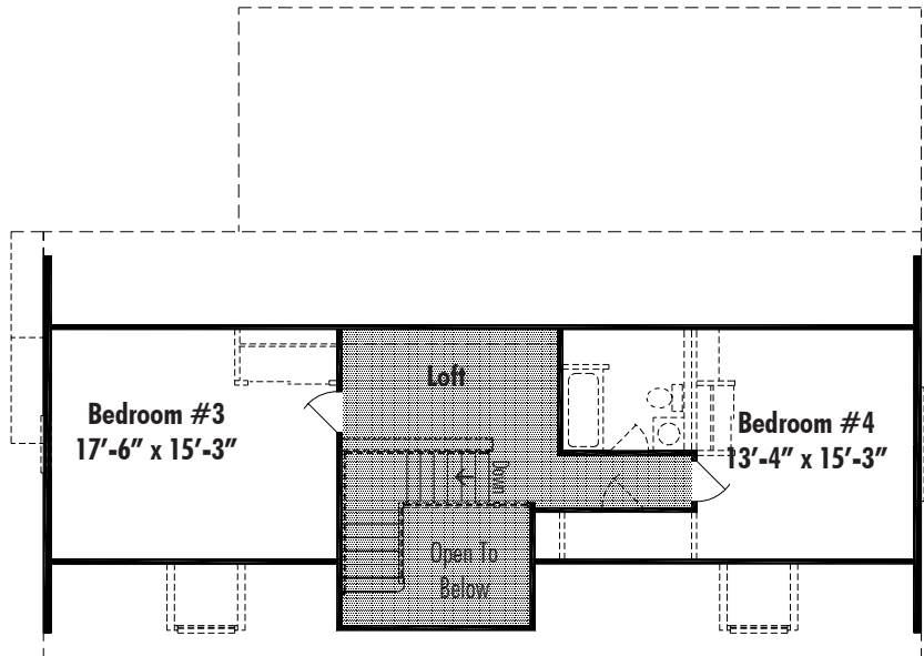
Layout C Front Balcony with Loft Second Floor Living Area 787 Sq. Ft.
