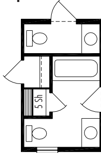
RPH2 Private Bath and Hall Half Bath
