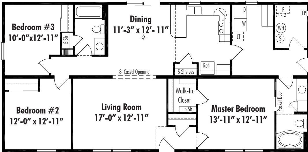
Millwood A.56 Crawl Space 27'-4" x 56', 1531 Sq. Ft. Living Area
