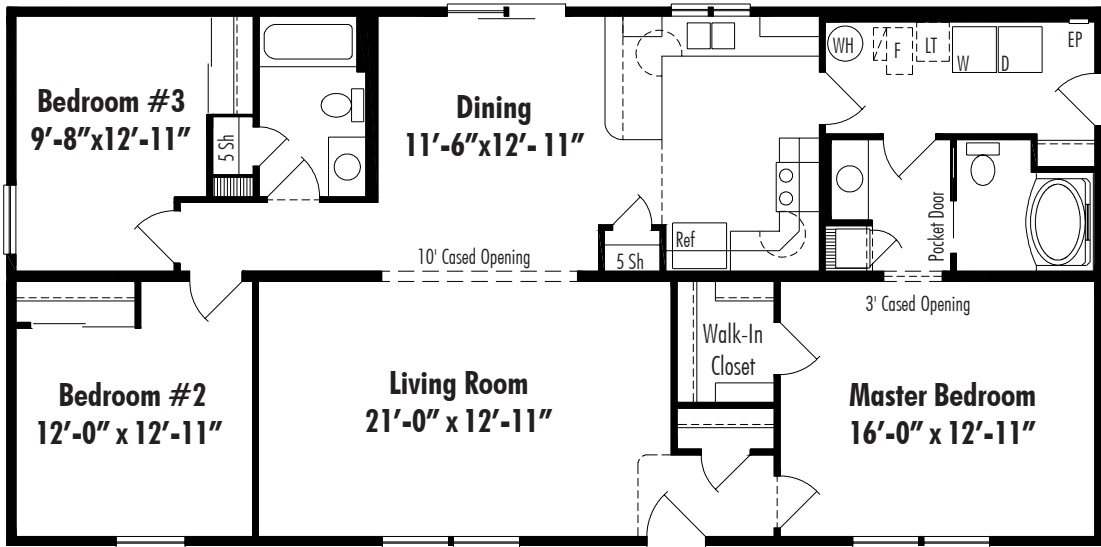
Millwood E.56 Crawl Space 27'-4" x 56', 1531 Sq. Ft. Living Area
